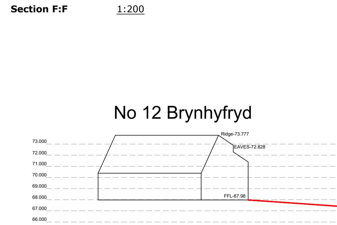
Section F:F 1:200
