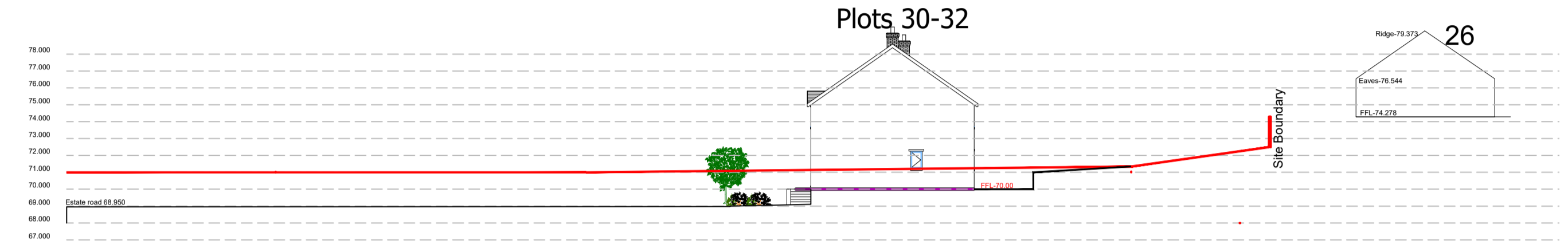
Section H:H 1:200
