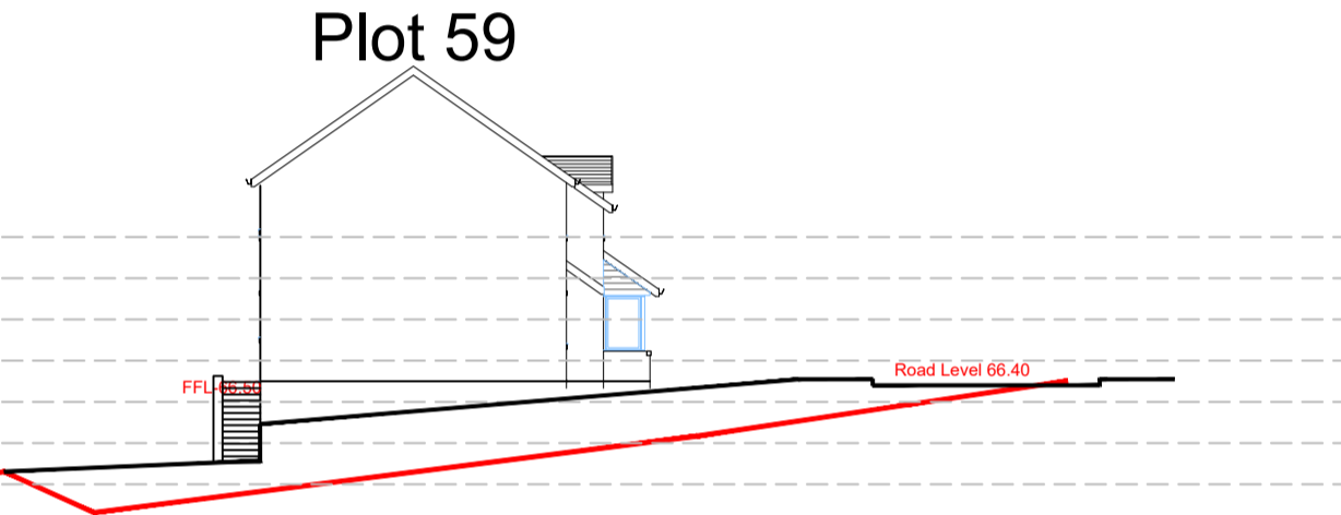
Section B:B 1:200
