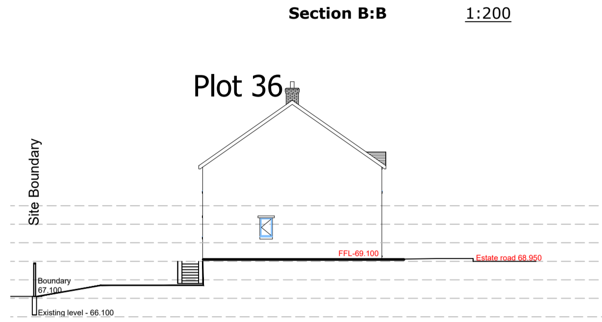
Section B:B 1:200
